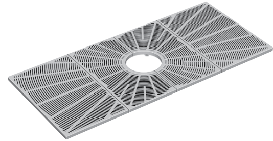
R-8813 • 48" x 107.75" Four-piece grate, 16" diameter expandable tree opening. Total grate length can be increased with additional end sections. .25" slot openings. Available with 20" and 24" diameter tree opening. 636 pounds per set. R-8813 is also a Los Angeles approved grate. Special frames and/or supports required.
