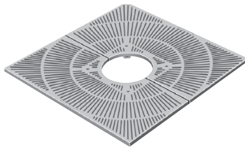
R-8714-A • 60" x 60" 18" diameter tree opening. .375" slot openings. Four 1" diameter holes for staking tree. 520 pounds per set. Available with light openings. R-8714-ALA Order as R-8714-ALA for Los Angeles approved grate.
