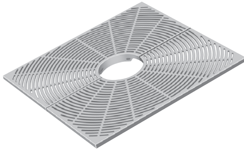
R-8712 • 60" x 60" 16" diameter expandable tree opening. .375" slot openings. 580 pounds per set. Available with light openings.
