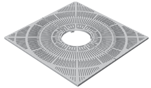
R-8707 • 60" x 60" 18" diameter expandable tree opening. Available with cast 24" tree opening. .25" slot openings. 525 pounds per set. Available with light openings. R-8707-LA Order as R-8707-LA for Los Angeles approved grate. Only available with 18" diameter tree opening.
