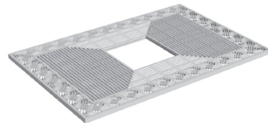
R-8850 • 48" x 72" 2-piece grate with 18" square tree opening. 380 pounds per set.
