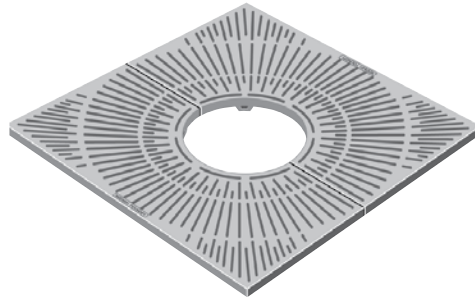
R-8706-1A • 48" x 48" 18" diameter expandable tree opening. .25" slot openings (Available with light openings, order as R-8706-A ). 330 pounds per set. R-8706-1A is also a Los Angeles approved grate. Available with light openings.
