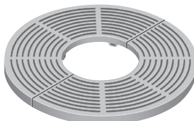
R-8881 • 30" Round 12" diameter expandable tree opening. .25" slot openings. 84 pounds per set.
