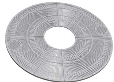
R-8883 • 96" Round 28" diameter tree opening. .25" slot openings. 960 pounds per set. Supplied in 12 sections. Support at section joint is required — furnished by installer. Available with light openings.
