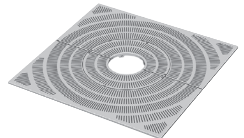
R-8718-A • 72" x 72" Four-piece grate, 16" diameter tree opening, insert grate removes for 36" diameter tree opening. .25" slot openings. 850 pounds per set. Available with light openings.
