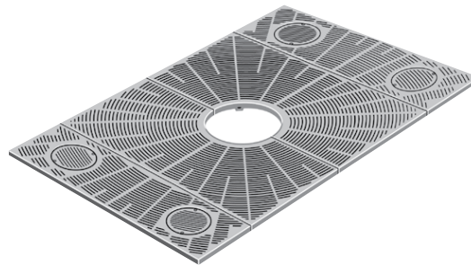
R-8816 • 60" x 95.75" Four-piece grate, 18" diameter expandable tree opening. .25" slot openings. 706 pounds per set. Available in 16", 24" and 36" tree openings. Also available with no light openings.
