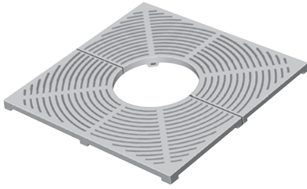
R-8704 • 30" x 30" 12" diameter expandable tree opening. .25" slot openings. 100 pounds per set. R-8704 is also a Los Angeles approved grate.
