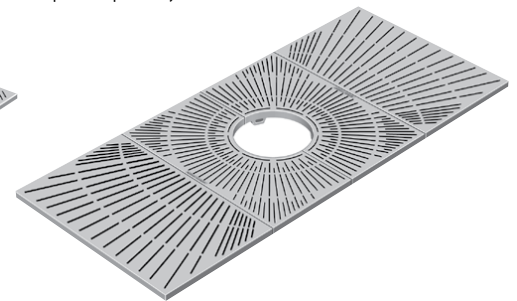
R-8817 • 48" x 108" Four-piece grate, 18" diameter expandable tree opening. .25" slot openings. 685 pounds per set. Available with light openings.
