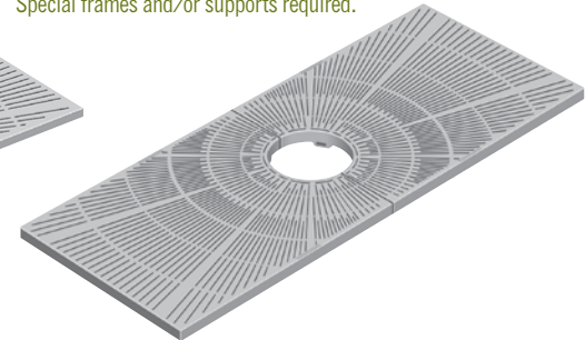
R-8815-B • 48" x 120" Two-piece grate, 18" diameter tree opening. .25" slot openings. 762 pounds per set. (Available as 48" x 96" 2-piece grate with 18" and 26" diameter tree opening, order as R-8815-A . 646 pounds per set.)
