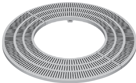
R-8871-1 • 60" Round 32" diameter expandable tree opening. .25" slot openings. 336 pounds per set. Available with light openings. (Available with 16" diameter expandable tree opening, order as R-8871 . 376 pounds per set.) R-8871-1 is also a Los Angeles approved grate.
