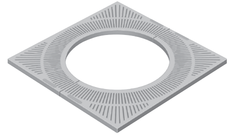
R-8719 • 48" x 48" 32" diameter expandable tree opening. 302 pounds per set.
