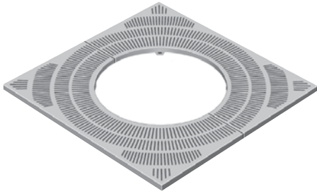
R-8717 • 60" x 60" 36" diameter tree opening. .25" slot openings. 440 pounds per set. (Available with removable insert grate and 16" tree opening, order as R-8717-A . 580 pounds per set.) R-8717 is also a Los Angeles approved grate.
