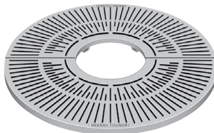
R-8834 • 36" Round 12" diameter expandable tree opening. .25" slot openings. 126 pounds per set.
