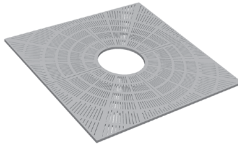
R-8784 • 95.125" x 95.125" 26" tree opening. .25" slot openings. 4-piece grate. 1588 pounds per set. Support at section joint is required — furnished by installer.
