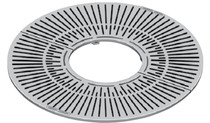
R-8830-A1 • 48" Round 18" diameter expandable tree opening. .25" slot openings. 252 pounds per set. (Available with light openings, order as R-8830-1 . 268 pounds per set.) R-8830-A1 or R-8830-1 are also Los Angeles approved grates.
