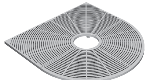
R-8939 • 72" Combo 16" diameter expandable tree opening. .25" slot openings. 661 pounds per set. Available with light openings.
