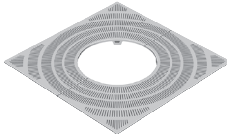
R-8718 • 72" x 72" 36" diameter tree opening. .25" slot openings. 750 pounds per set. Available with light openings. R-8718 is also a Los Angeles approved grate.
