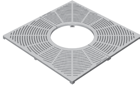
R-8704-A • 36" x 36" 16" diameter expandable tree opening. .25" slot openings. 115 pounds per set. Available with corner light openings. 9.5" x 1" grate or 7.875" x .75" lid. R-8704-A LA Order as R-8704-A LA for Los Angeles approved grate.
