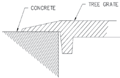
RETROFIT DETAIL
