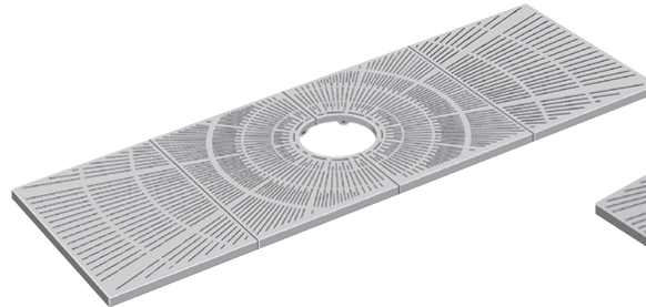
R-8815 • 48" x 144" Four-piece grate, 18" diameter tree opening. .25" slot openings. 928 pounds per set. Available with 24" diameter tree opening. (Available as 48" x 120" 4-piece grate with 18" diameter tree opening, order as R-8815-B4 . 898 pounds per set).
