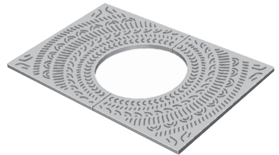
R-8819 • 48" x 72" 30" diameter tree opening. .375" typical slot openings. 390 pounds per set.
