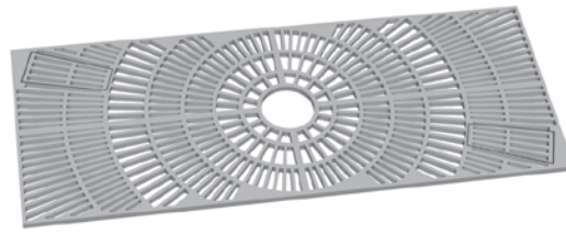
R-8806-1A • 48" x 120" Four-piece grate, 12" diameter expandable tree opening. Bolted light opening grates (9" x 19" x 6") for use with sub-grade lighting. Support at section joint is required — furnished by installer. Parented with two light openings only. 720 pounds per set.
