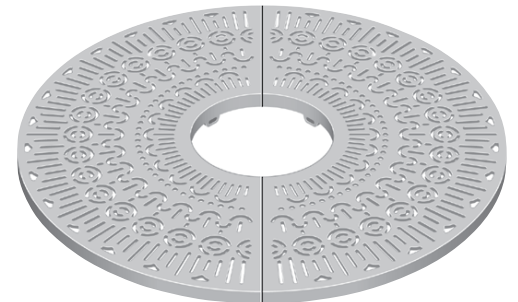
R-8874 • 48" Round 14" diameter tree opening. .375" typical slot openings. 220 pounds per set. Available with light openings. R-8874 is also a Los Angeles approved grate.
