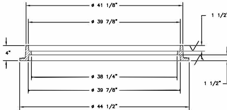
RING SECTION
